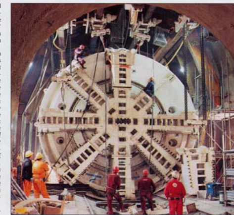
Regular servicing keeps the boring machines cutting their way towards France. 415V mobile plant connections are made by industrial plug and socket connections; a requirement of TML's site manager was that these could be repaired on the job.
